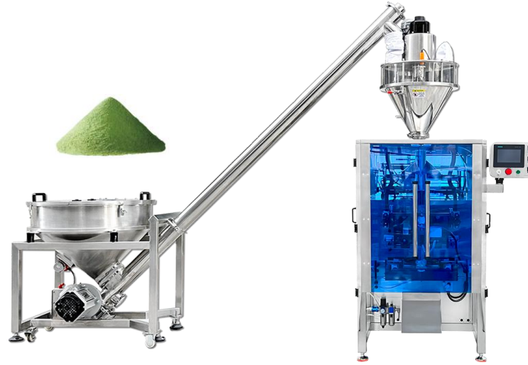
Powder lifter + powder meter + VFFS
