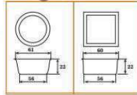
100-Cups Mix Cake Pan (Teflone Coating)
